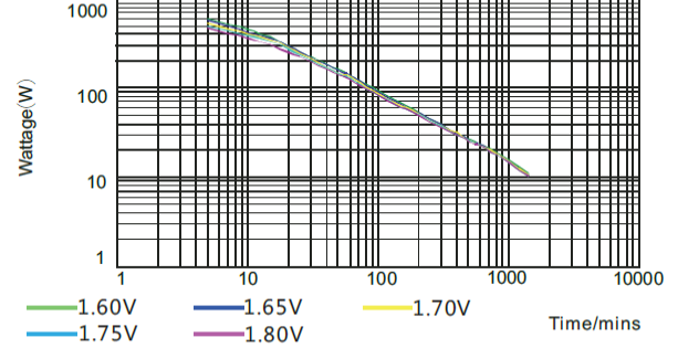
Constant Power Discharge
