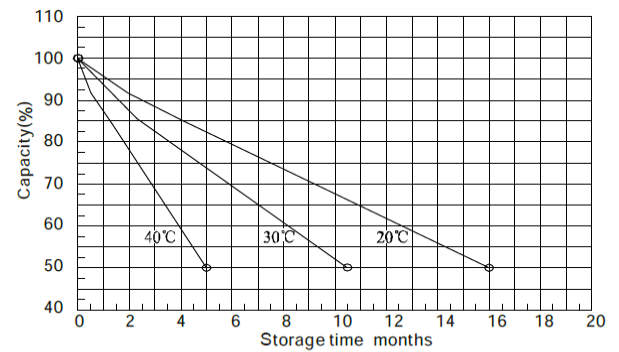
Self-discharge characteristic
