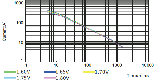
Constant Current Discharge
