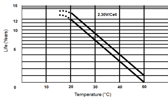
Temperature effects on Float Life
