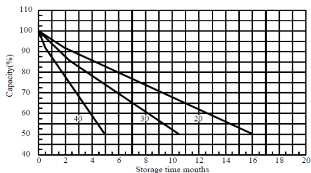
Self-discharge characteristic
