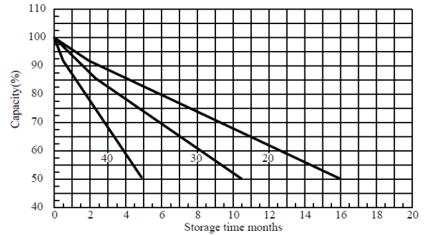
Self-discharge characteristic
